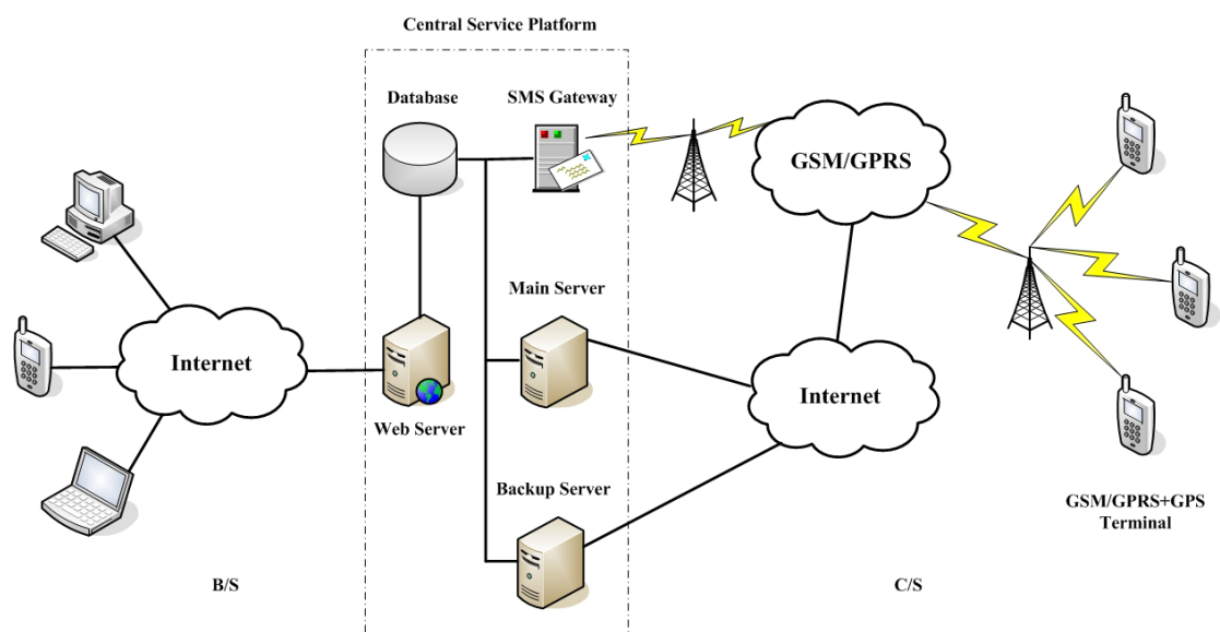
Figure 1: System architecture
